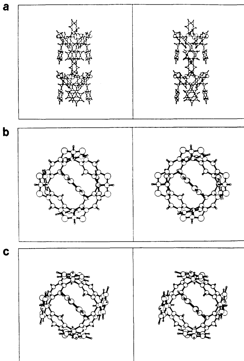
Figure 1. Different stereoviews of crystal structures of 2(16 \cdot C_6H_6) and 16 \cdot C_6H_6 : (a) side view of 2(16 \cdot C_6H_6) , (b) bowl-face view of 16 \cdot C_6H_6 , and (c) box-face view of 16 \cdot C_6H_6 .
