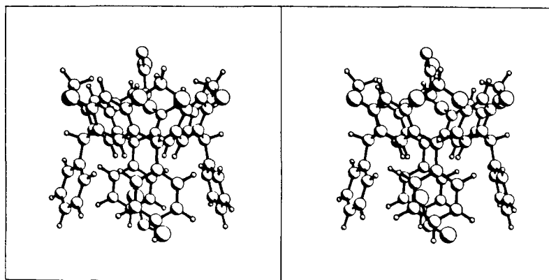
Figure 2. Side stereoview of 16 \cdot CH_3COCH_3 \cdot CH_2Cl_2 .
