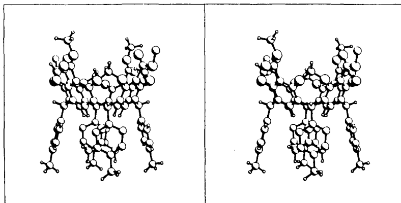
Figure 3. Side stereoview of 23 \cdot \text{CH}_3\text{COCH}_3 .
